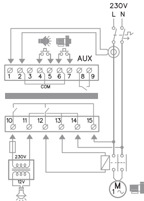
1-phase with contactor
